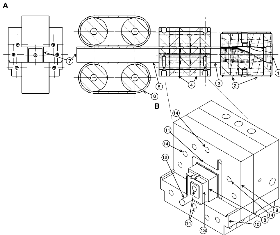
Fig. 11 Profile vacuum calibration and take-off. (A) Section view of calibration process: (1) melt enters profile die; (2) profile die stack; (3) molten profile extrudate; (4) calibrator (cools, shapes, and sizes extrudate); (5) solidified plastic; (6) puller; (7) orientation of profile. (B) Partially disassembled calibrator: (8) profile passing through calibrator; (9) upper calibrator stack; (10) lower calibrator stack; (11) upper vacuum channel; (12) lower vacuum channel; (13) core feature of lower calibrator; (14) cooling line.
