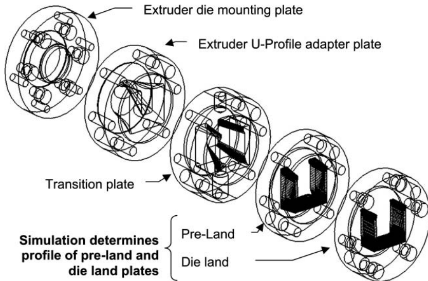
Fig. 12 U-Profile die plates designed with CFD simulation.
